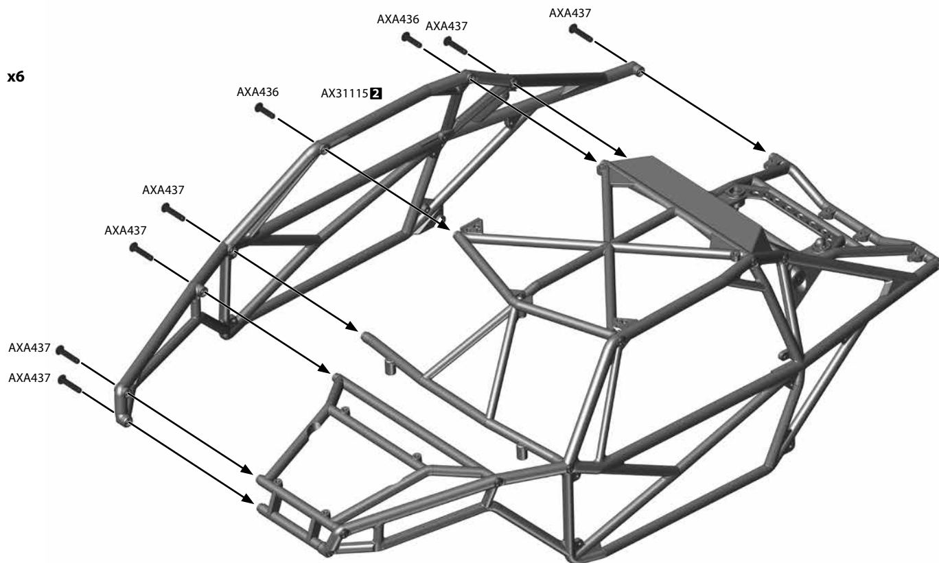
AXA437 M3x15mm
