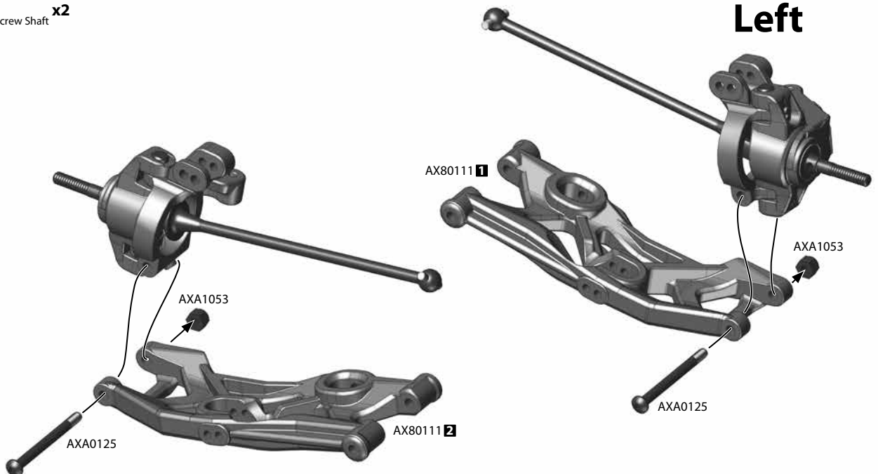
AXA1053 M3 Nylon Locking Hex Nut x2
