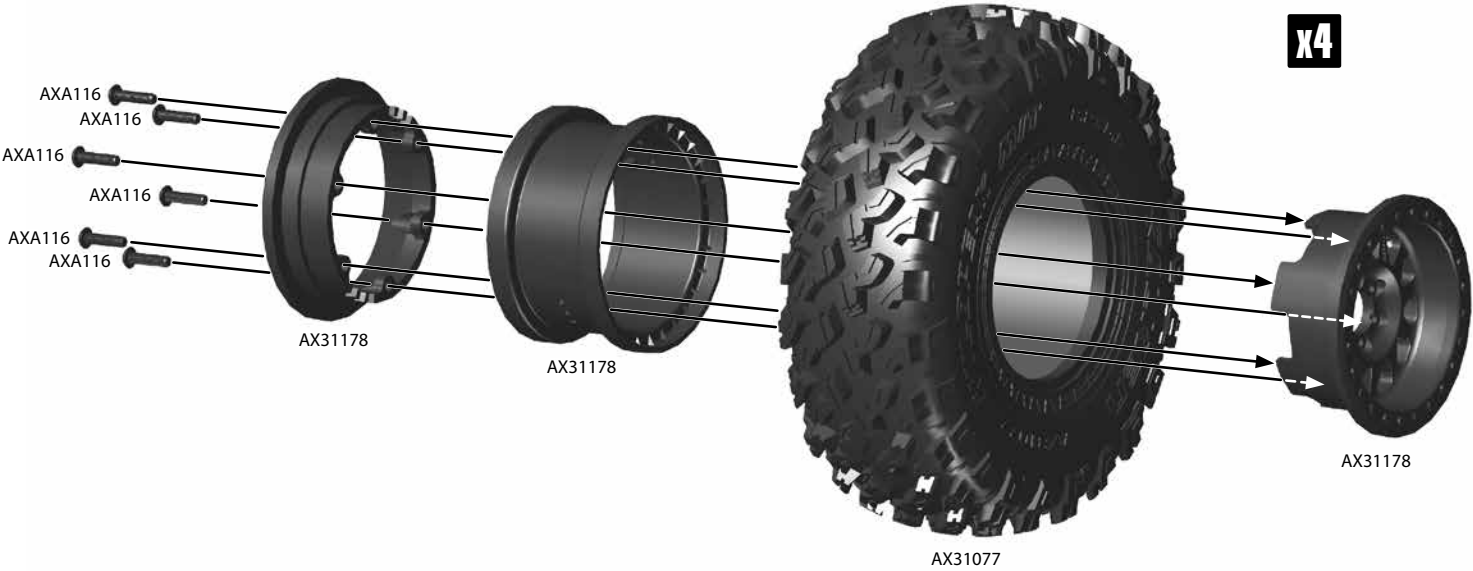
AXA116 M3x12mm x24
