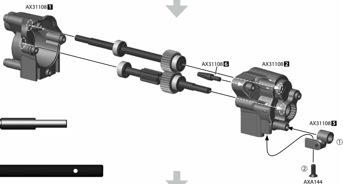
AX31129 2-Speed Hi/Lo Transmission Bottom Shaft (5x75mm) x1
