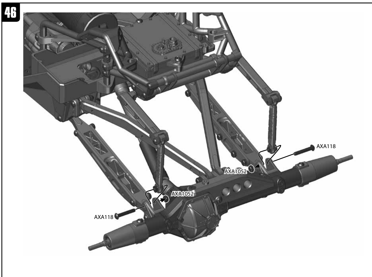
AXA1052 M3 Thin Nylon Locking Hex Nut x2
