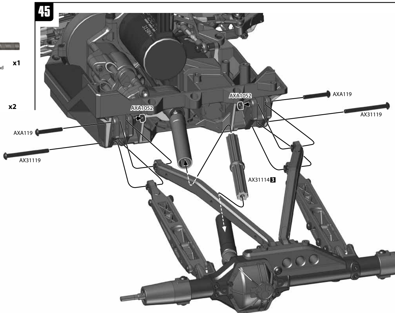
AXA119 M3x20mm x2
